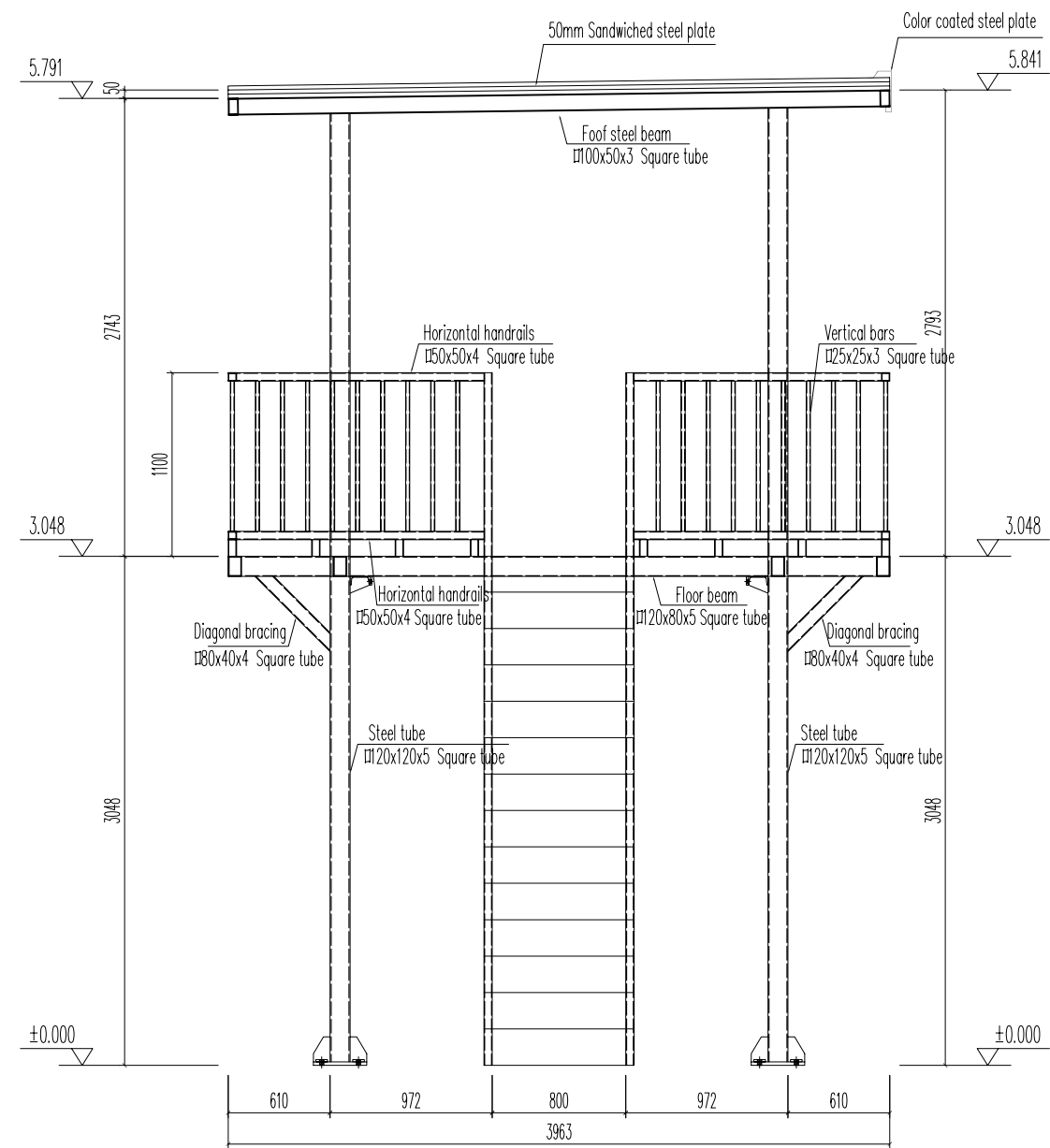
2 Axis Elevation
