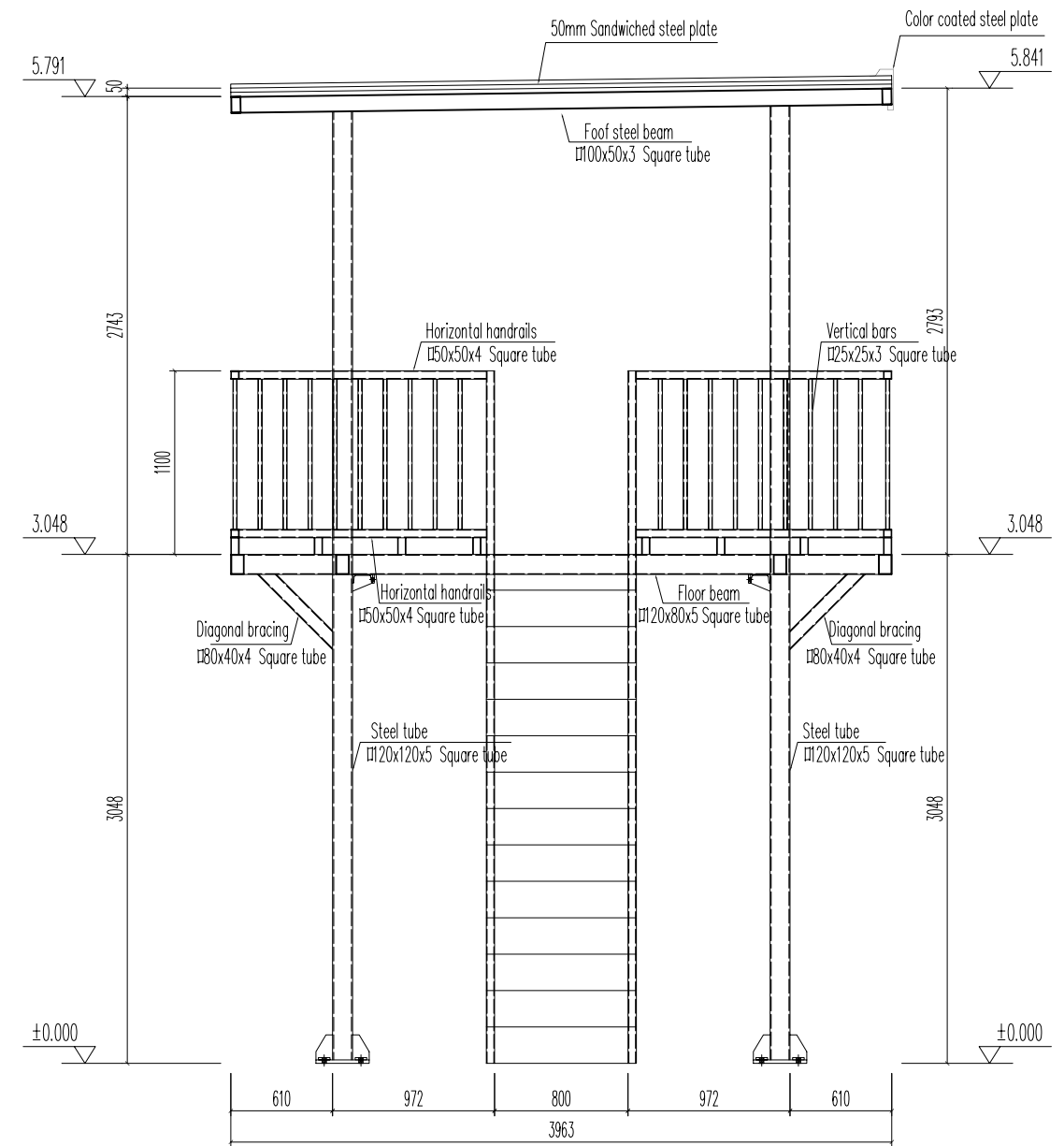
2 Axis Elevation
